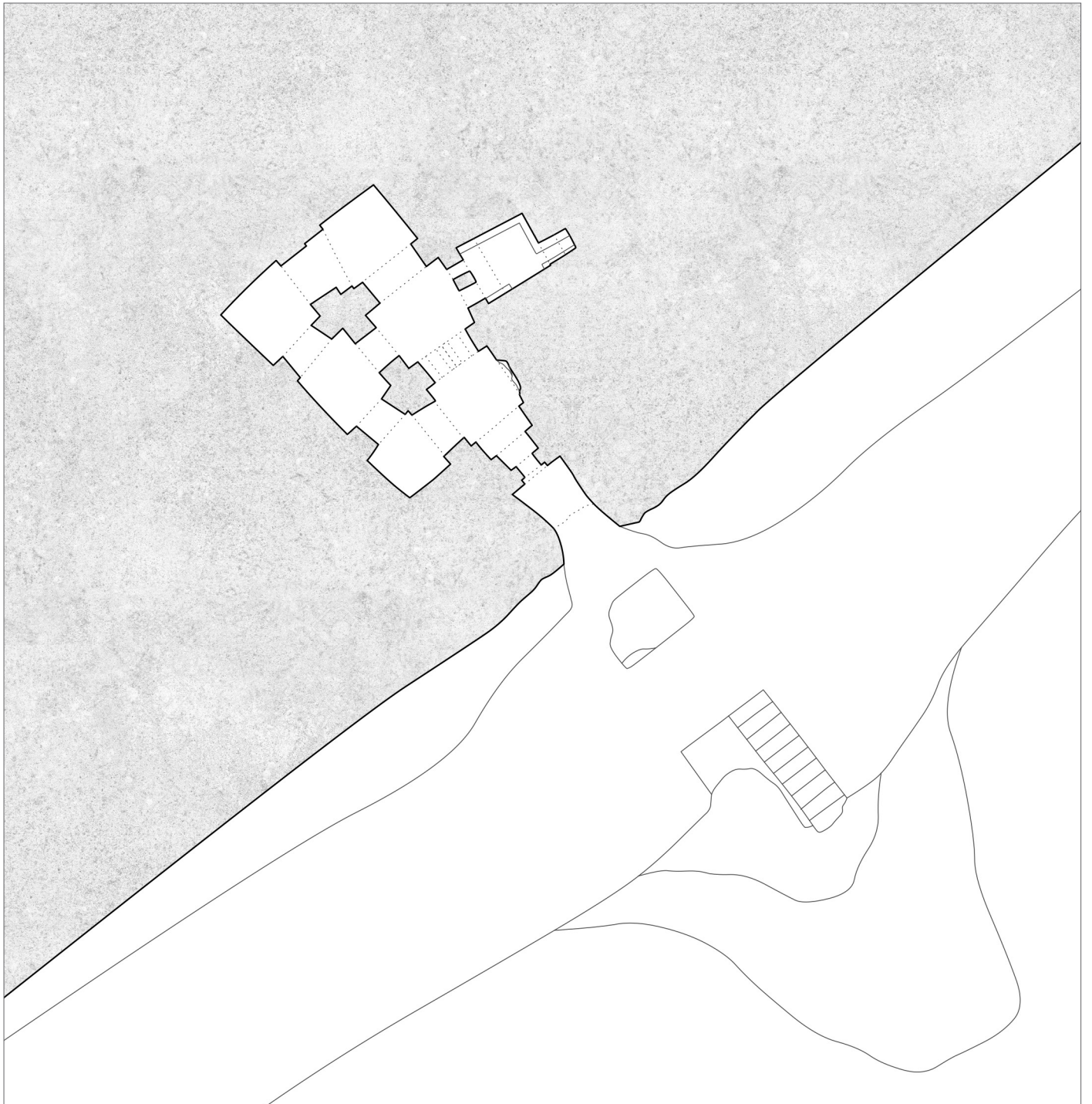
Sellase, Däbrä Tsion Ground Floor Plan (2020)
